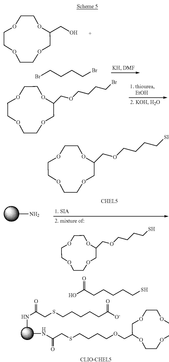
Example 6 Cesium Sensor
