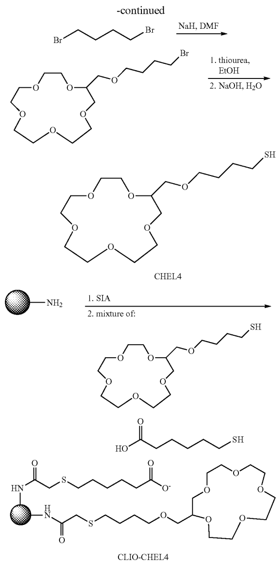
Example 5 Sodium Sensor
