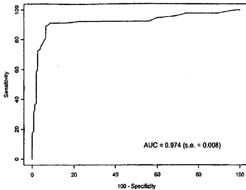
Figure 2: ROC curve for NT-proBNP (goat-6G11 assay).
