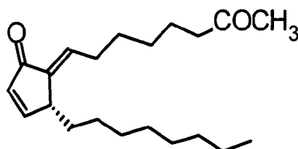
NEPP6
