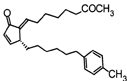
NEPP11
