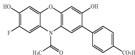
Compound 27
