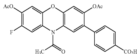
Compound 26
