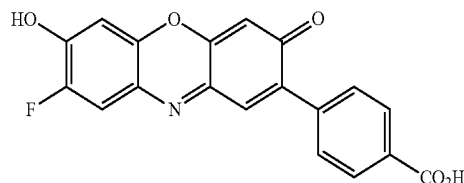
Compound 25
