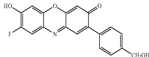
Compound 29
