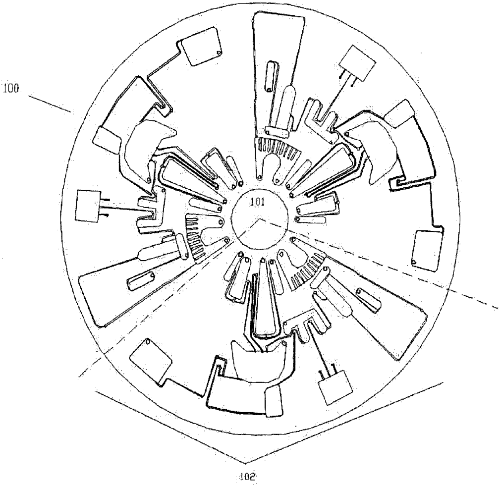
3-sample combined immunoassay and clinical chemistry disc
