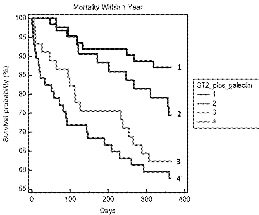
Figure 3: K-M Analysis of ST2 plus Galectin-3
