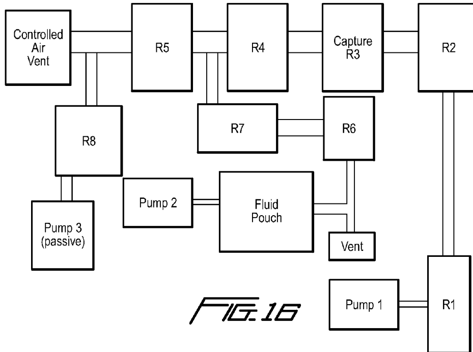
Fluidic Schematic for i-STAT immunocartridge
