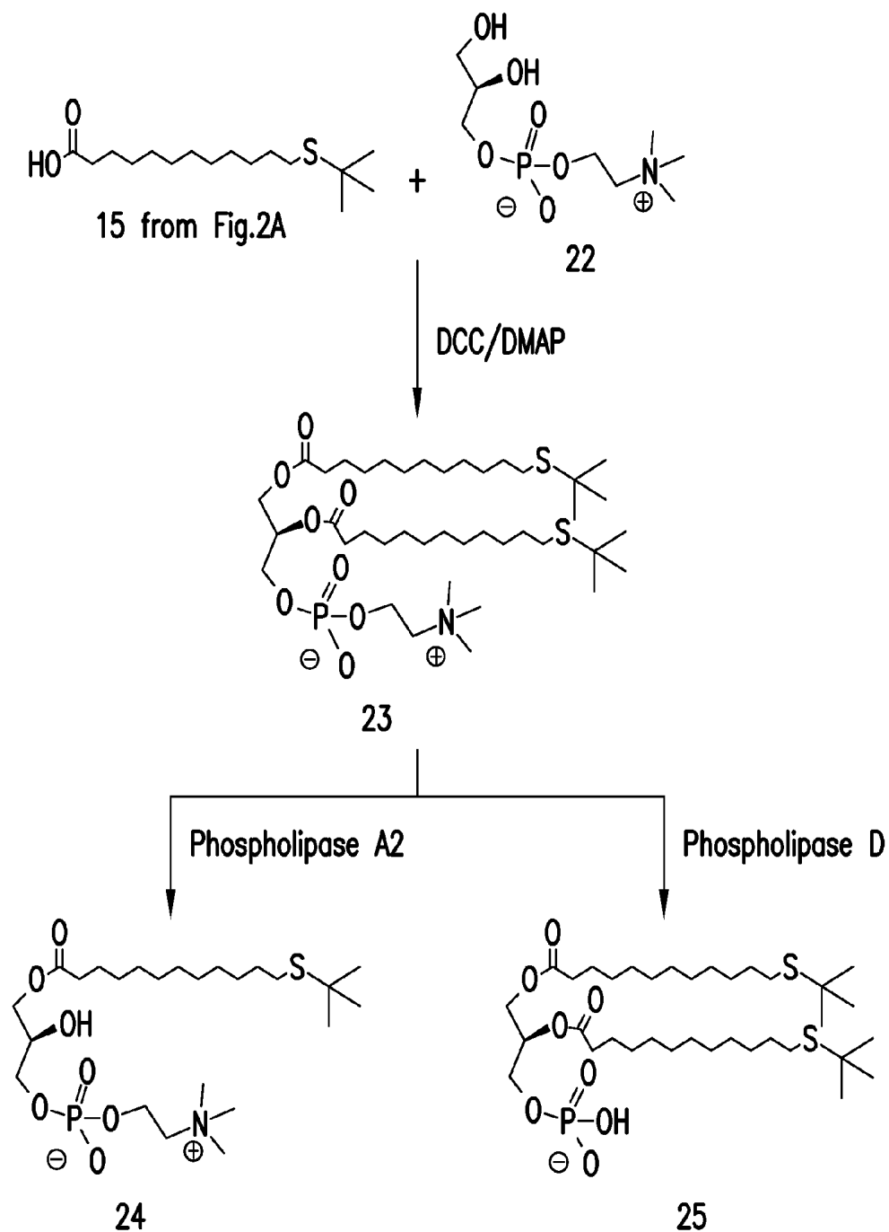
Synthesis of Typical Thiolated LPA Hapten
