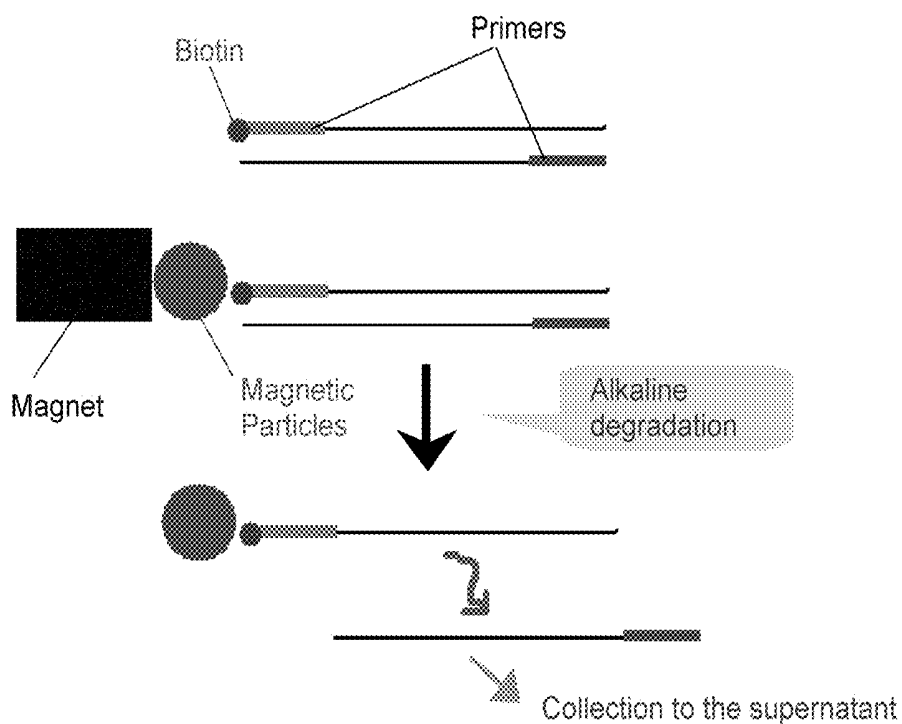
FIGURE: Making of the double-stranded DNA into a single strand using magnetic particles
