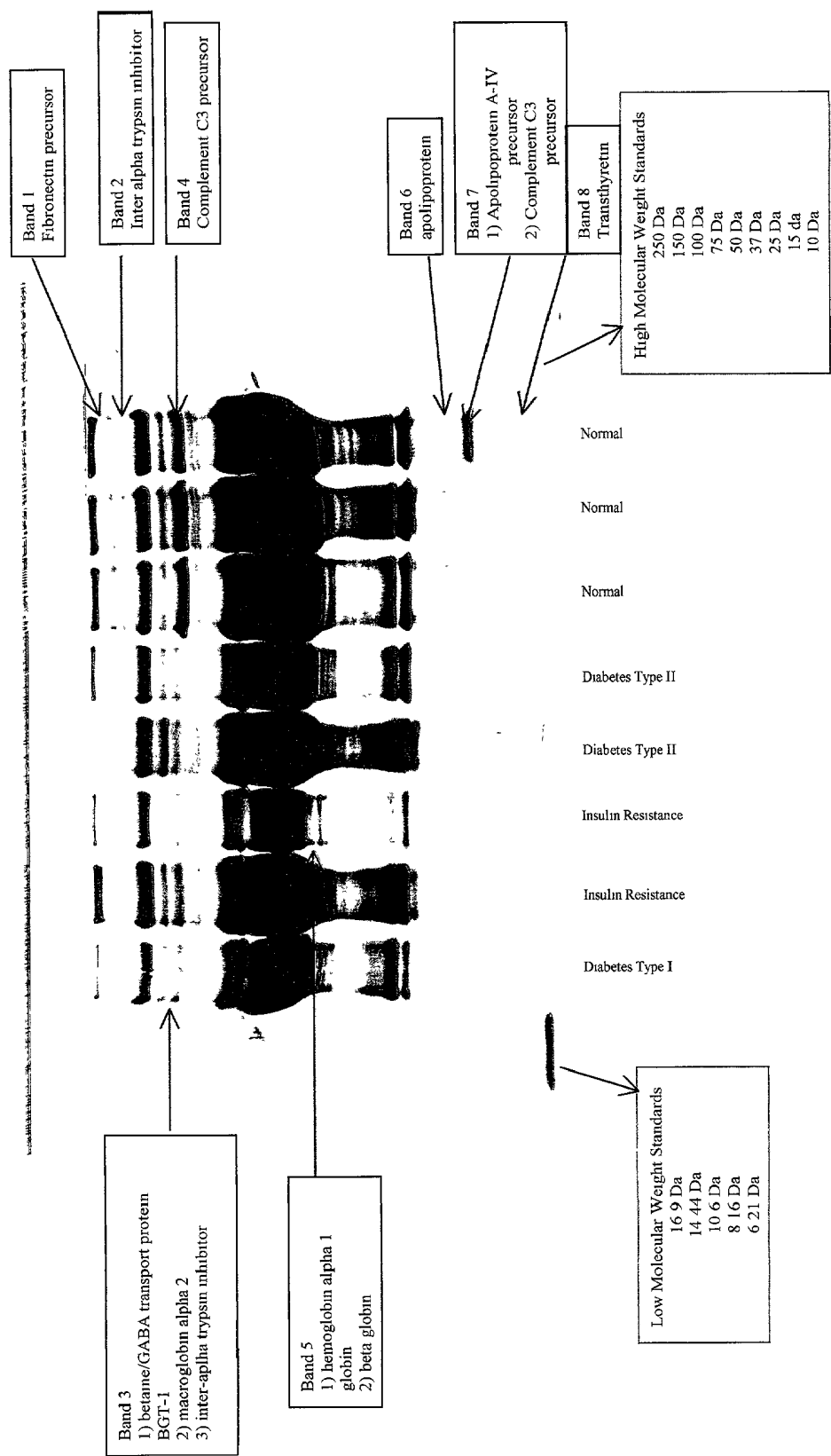
HiQ 1-(Elution) Insulin Resistance vs. Normal FIGURE 2
