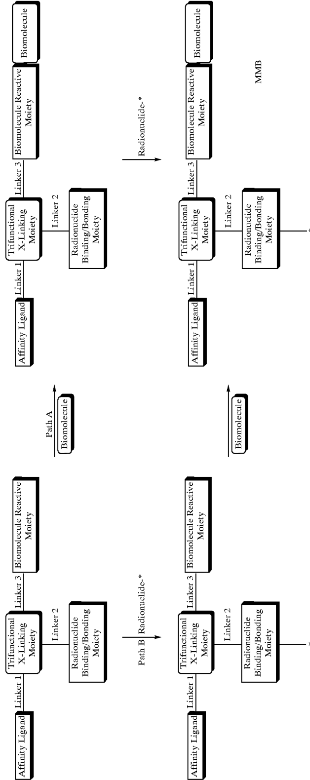
Scheme 2 Radiolabeling and Biomolecule Conjugation Paths
