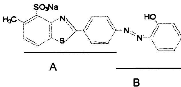
Benzothiazole analogue
