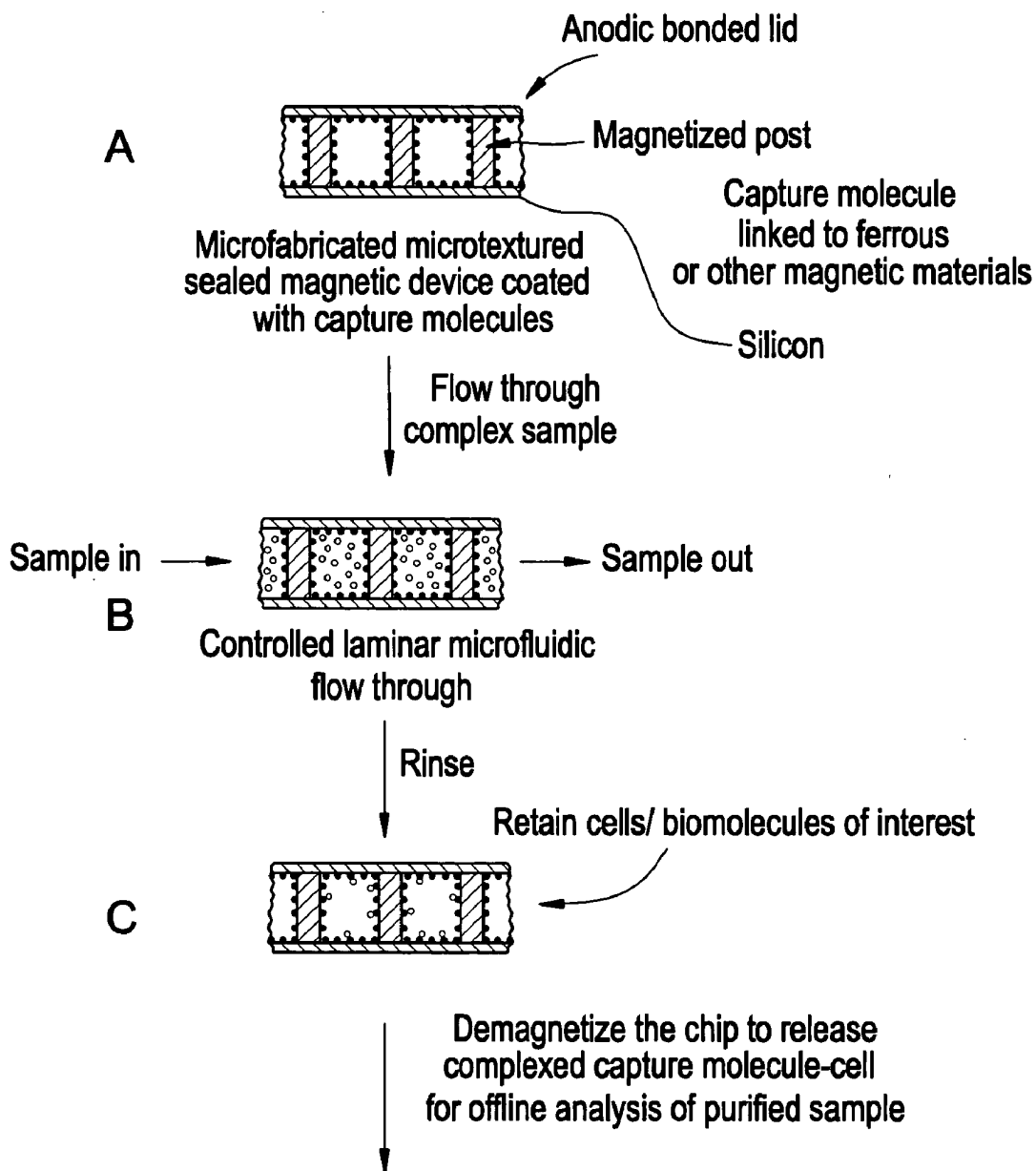
Cross-sectional view of device (A) and process flow for cell isolation and release for analysis (B & C)
