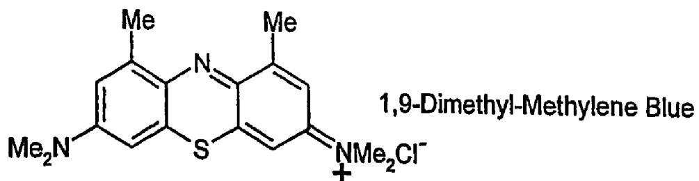
Methylene Blue
