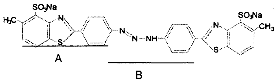
Thiazin yellow
