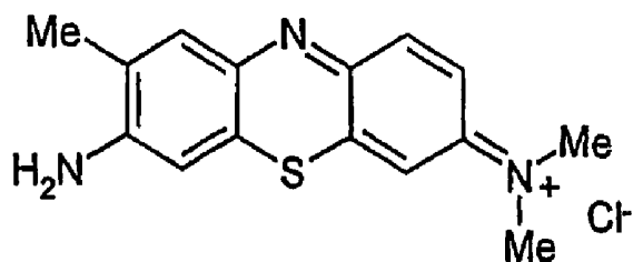
Tolonium Chloride
