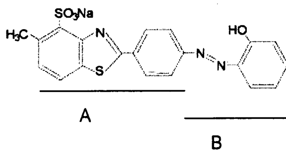
Benzothiazole analogue
