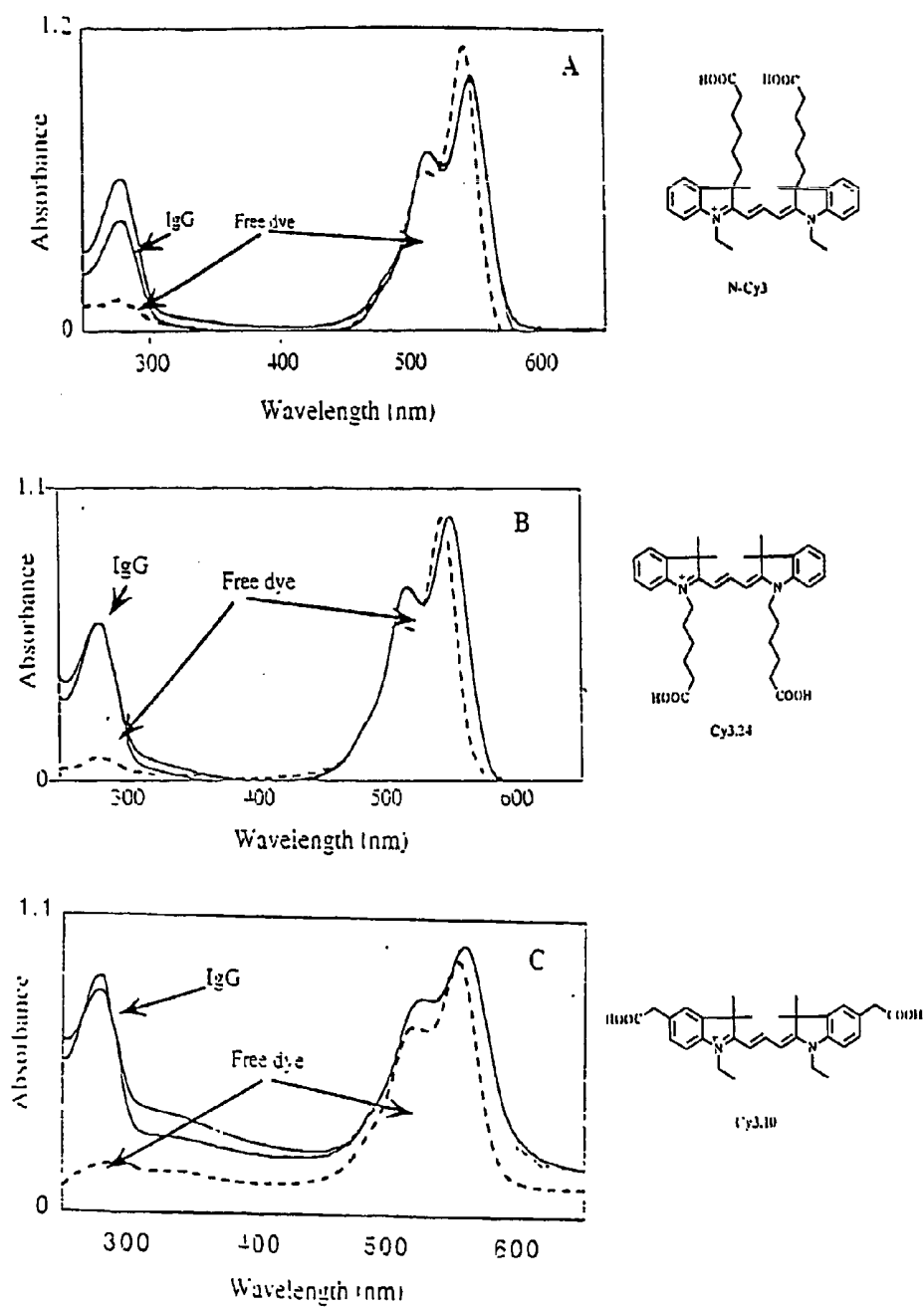
Absorption spectra of non-sulfonated Cy3 isomers and their antibody conjugates.
