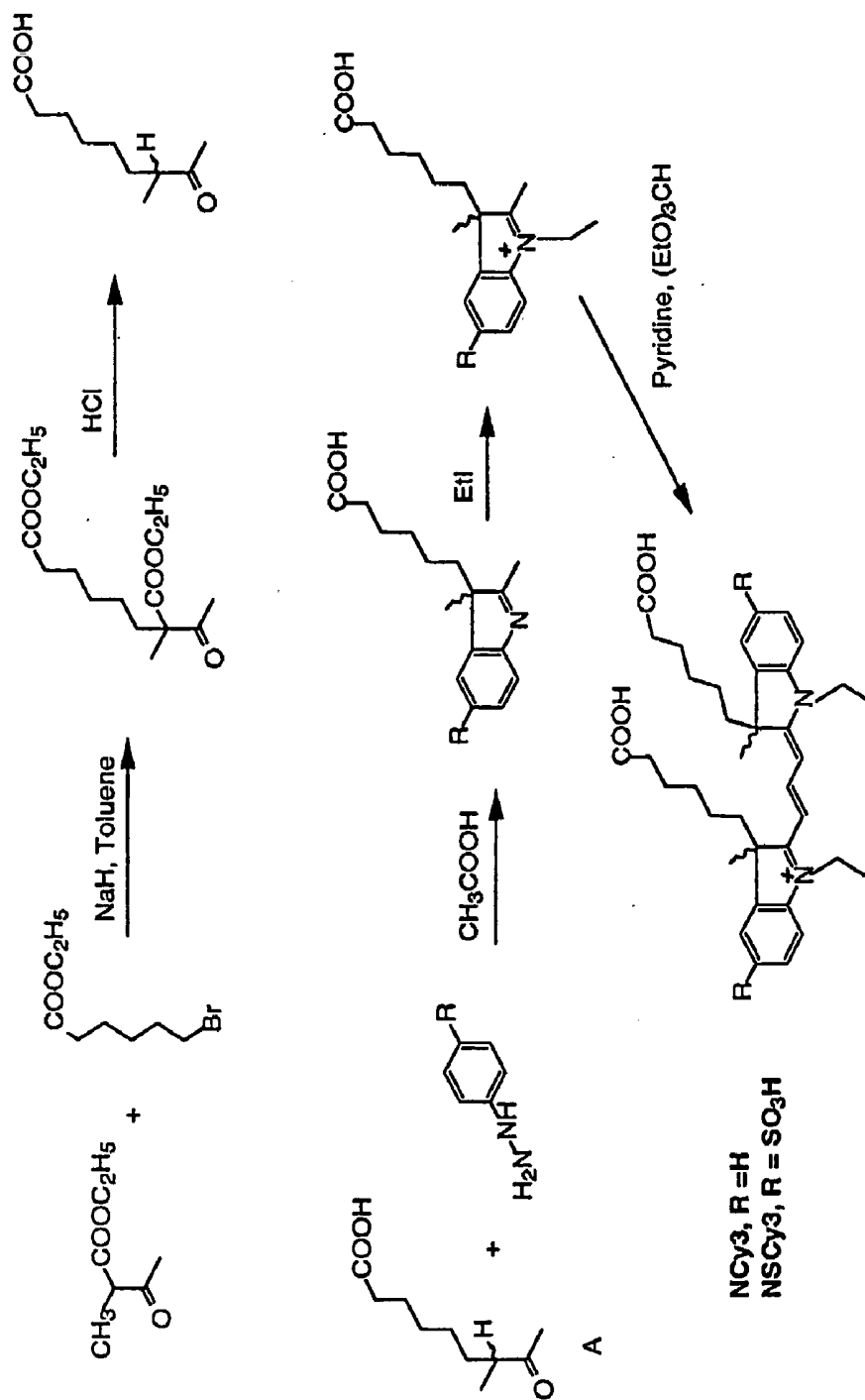
General scheme for the synthesis of functionalized ketone (A) and its cyanine dyes
