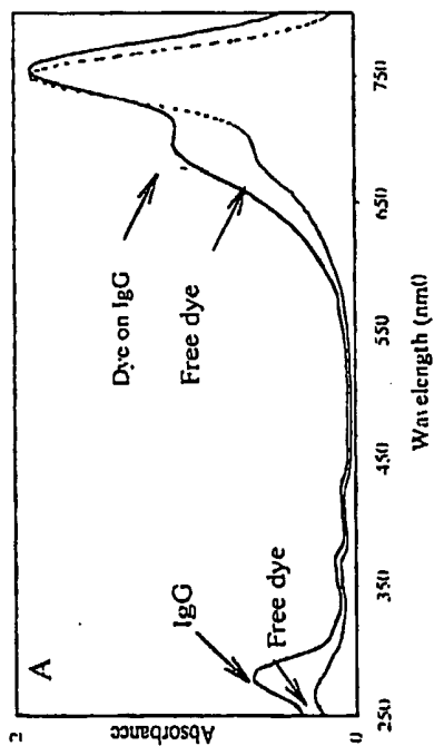
Absorption spectra of Cy7 18 and its protum conjugate
