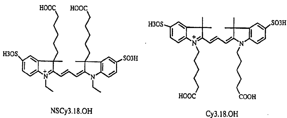
Sulfonated Cy3 dicarboxylic acid isomers
