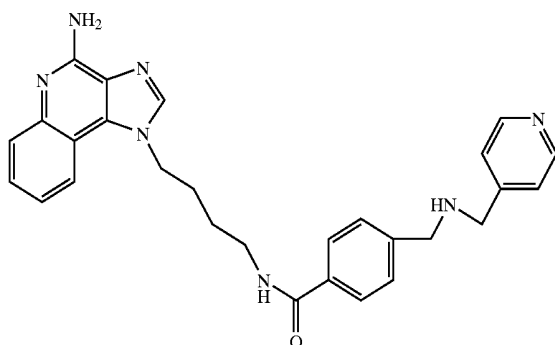
Compound II
