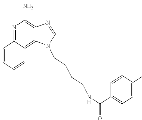
Compound I
