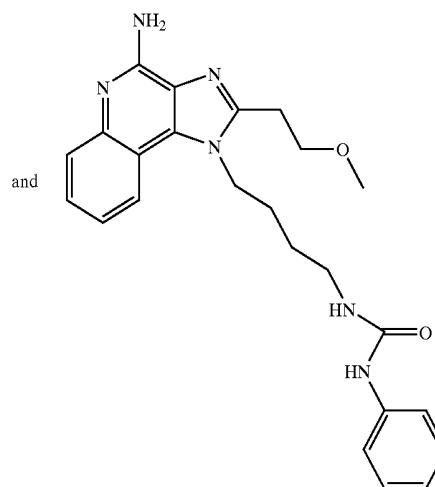
Compound VI
