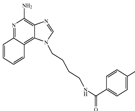
Compound I
