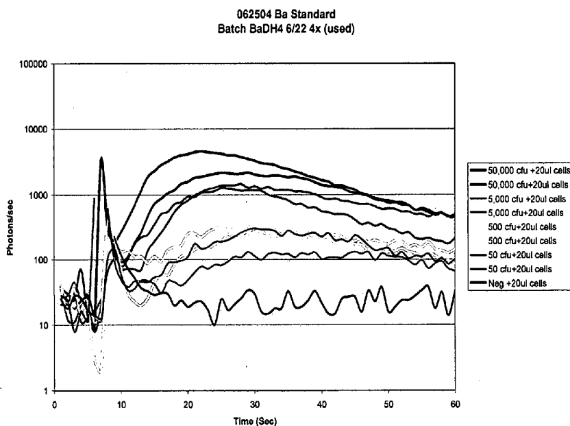
FIG. 106. Ba Standard with 20ul cell delivery. 50ul of Ba samples prepared in CO 2 (l) media and tested with 20ul B cells. Results indicate low background and an LOD of 50 cfu Ba (n=2).
