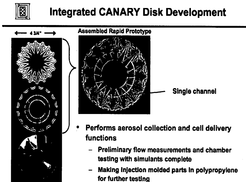
Figure 132. Automated CANARY bioaerosol sensor disk performs aerosol collection and CANARY B-cell storage and delivery functions.
