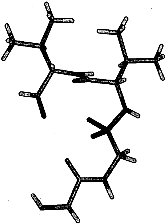
Gly-Gly-PO 2 - -NH-Val-Val
