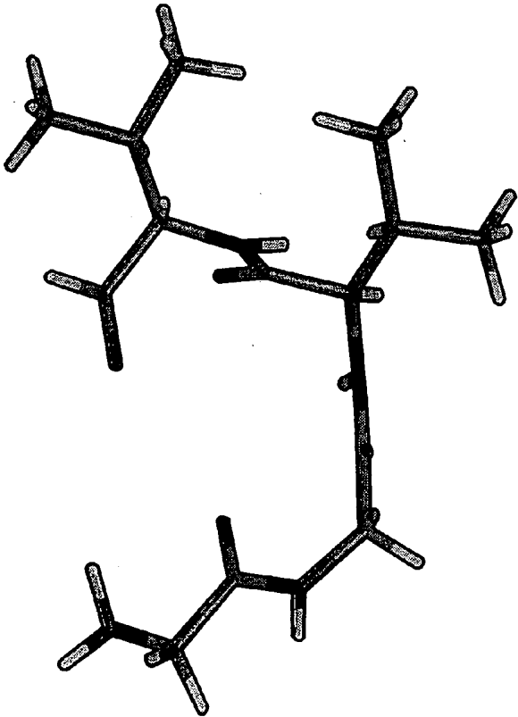
Gly-Gly-CO-NH-Val-Val
