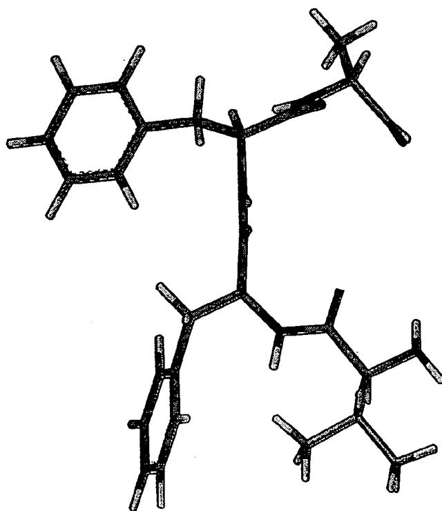
Val-Phe-CO-NH-Phe-Ala
