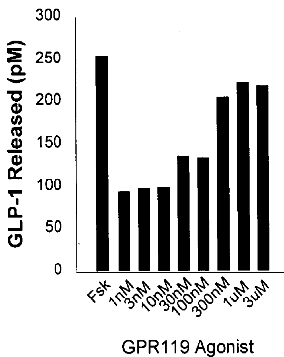
Figure 6. GPR119 Agonist Stimulates GLP-1 Secretion in GLUTag Cells
