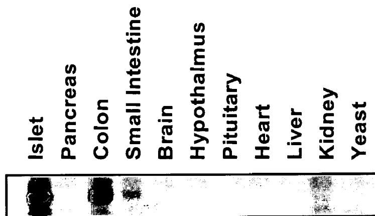
Figure 3. Expression of GPR119 in Gut
