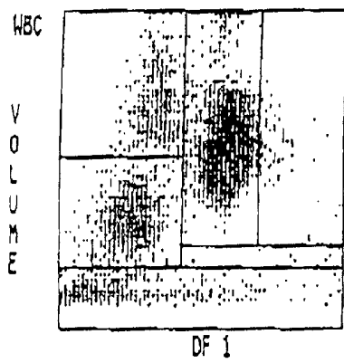
1-Butanesulfonic acid, sodium Lyse D.C. Volume vs. Light Scatter
