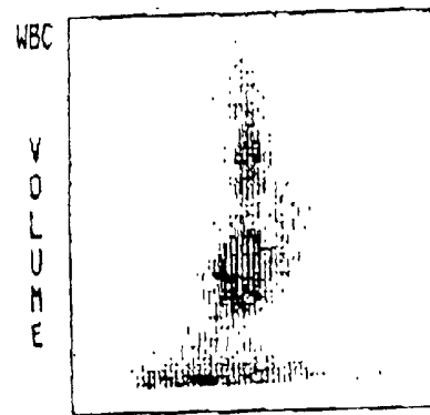
DF 3 COULTER Scatterpak Reagent D.C. Volume vs. Opacity
