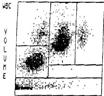
DF 1 CDS-5 PD Reagent Set D.C. Volume vs. Light Scatter
