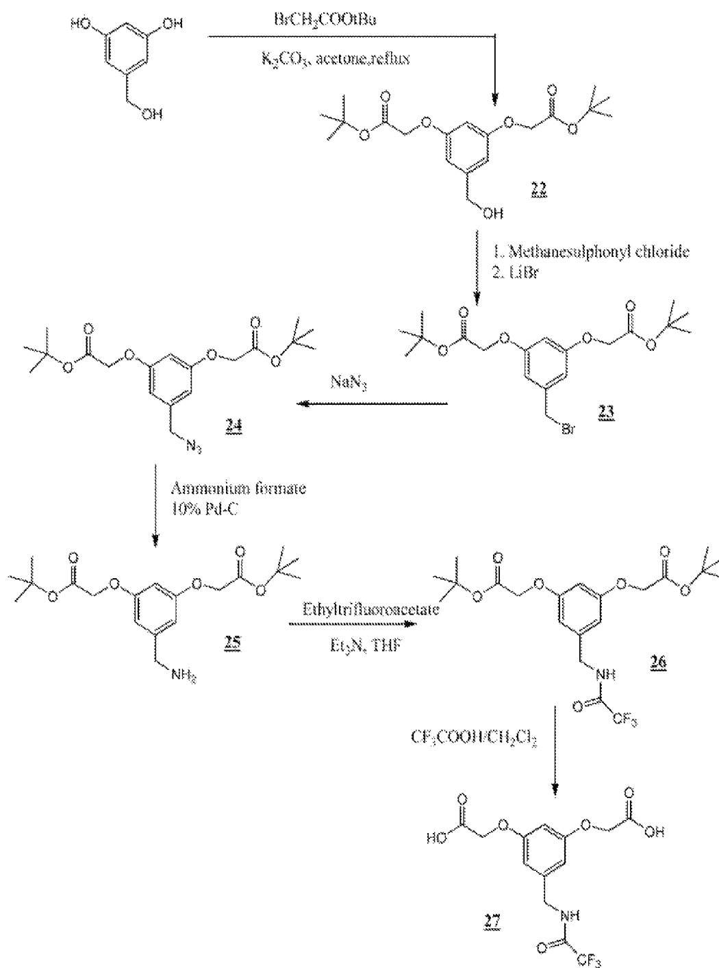
Aromatic trifluoroacetamido protected linker
