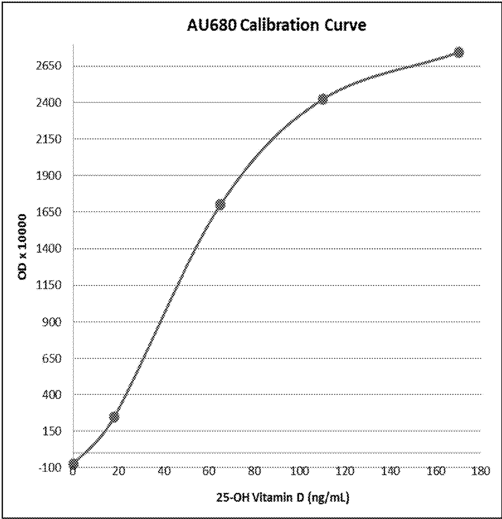
Figure 1. A typical calibration curve on AU680
