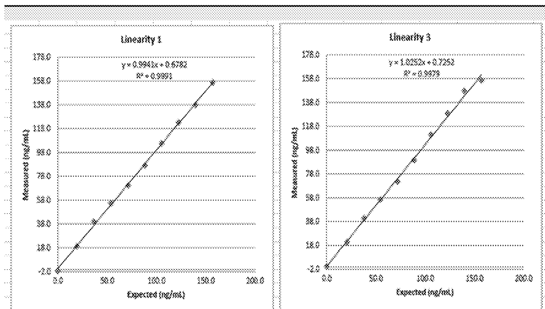
Assay linearity on AU 680 analyzer
