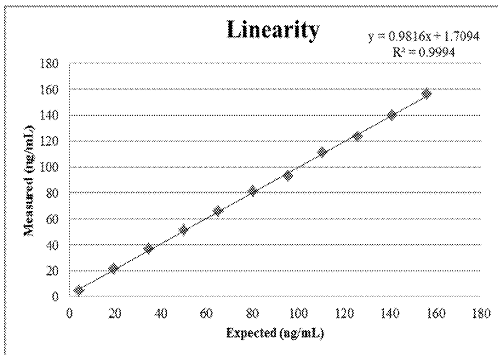
Figure 7. Linearity test results
