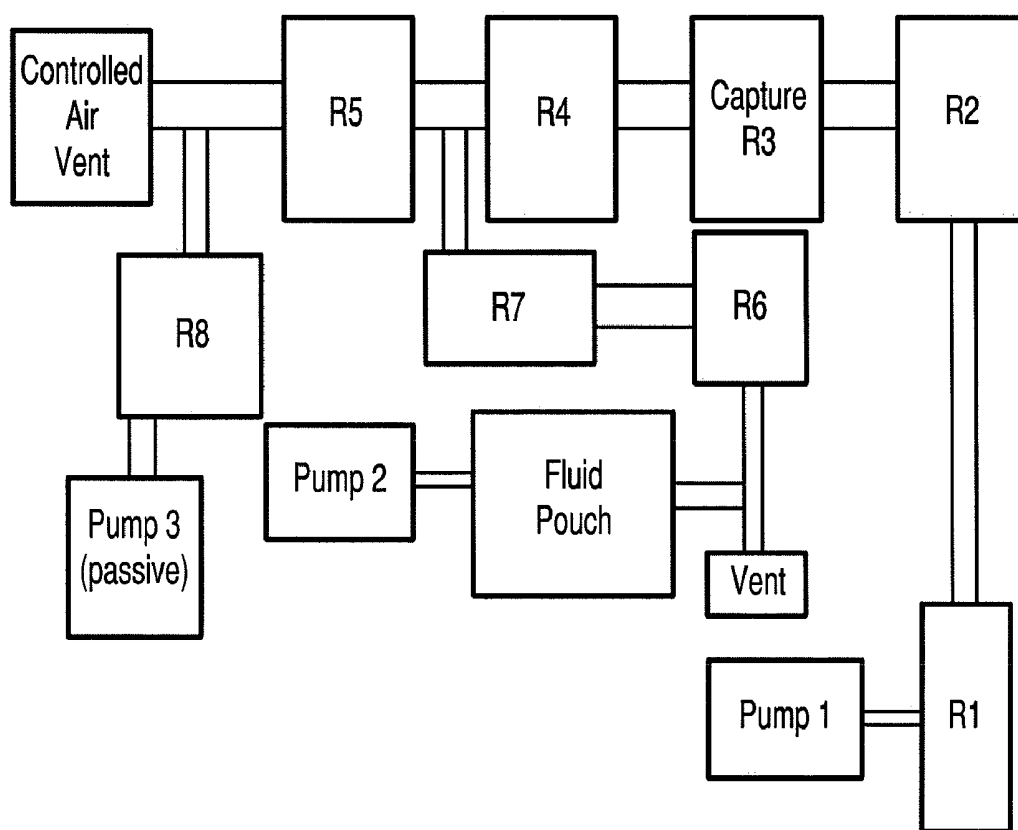
Fluidic Schematic for i-STAT immunocartridge
