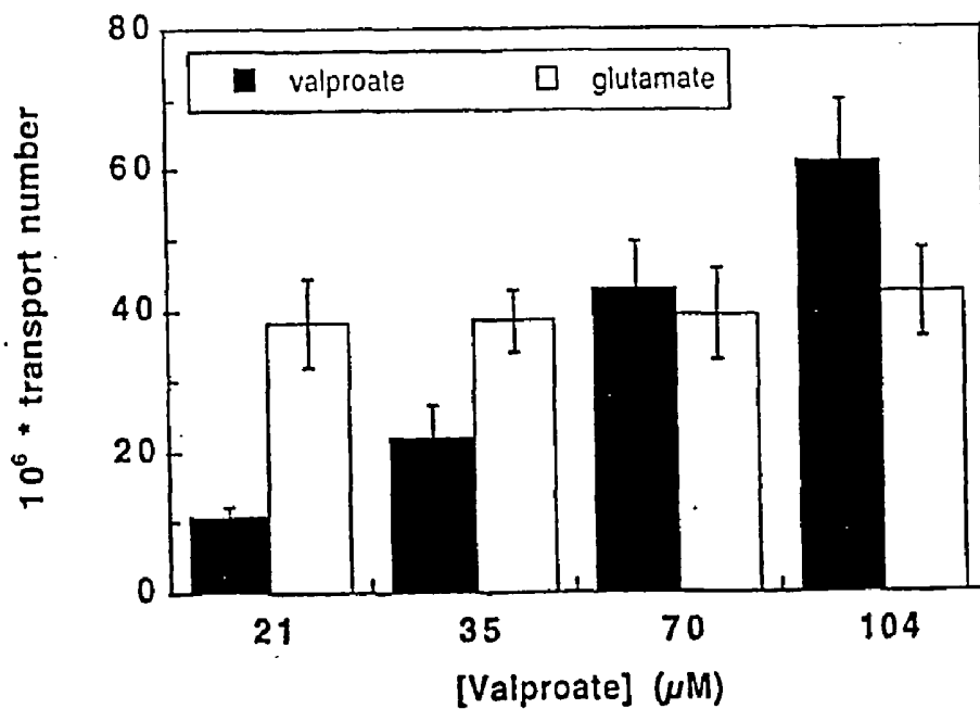
Valproate and glutamate transport numbers at 24 hours
