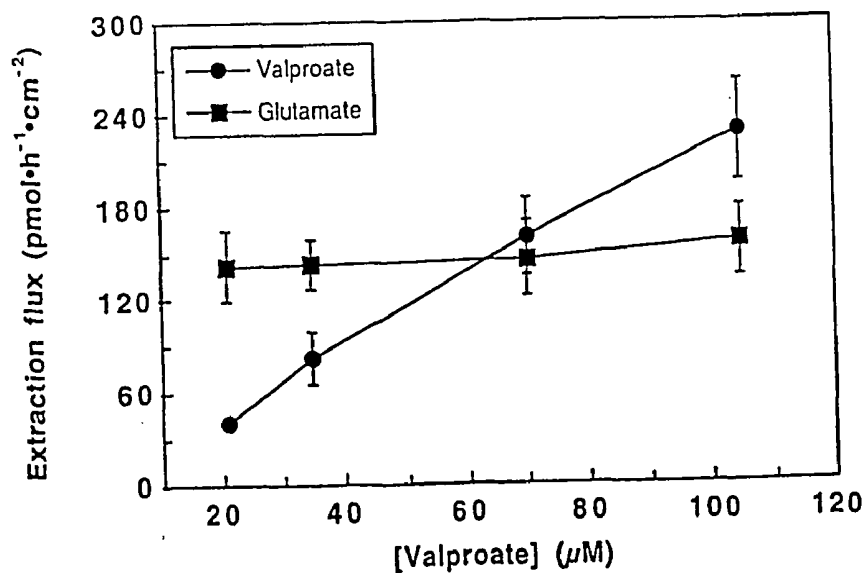
Extraction fluxes of Valproate and Glutamate at 24 hours
