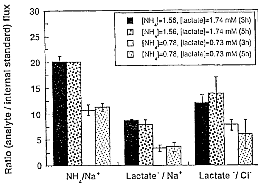
Extraction ratios of the analytes with respect to Na + and Cl -
