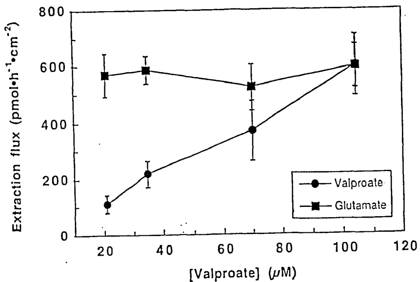
Extraction fluxes of Valproate and Glutamate at 5 hours
