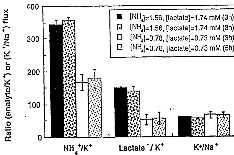
Extraction ratios of analytes with respect to K + and of K + with respect to Na +
