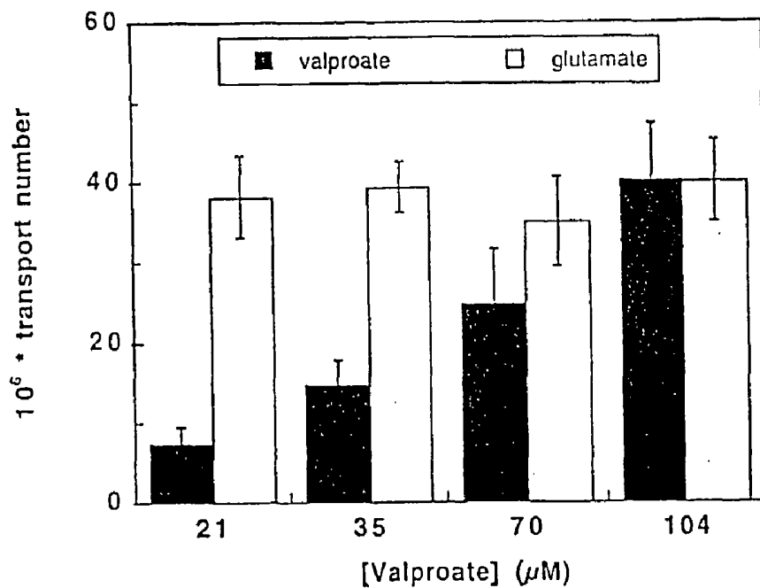
Valproate and glutamate transport numbers at 5 hours
