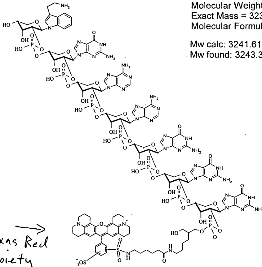
Figure 20 - structure and Mass Spec for TR-90-p-RNA Conjugate
