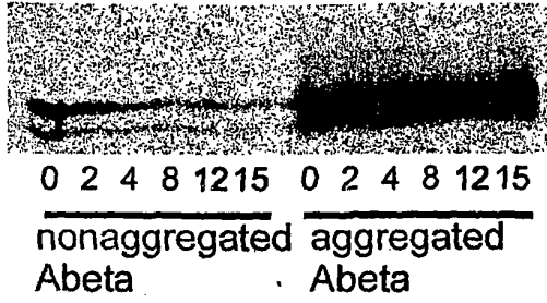
ONOO Treatment of nonaggregated and aggregated Abeta
