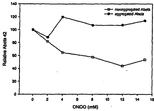
ONOO Treatment of nonaggregated and aggregated Abeta
