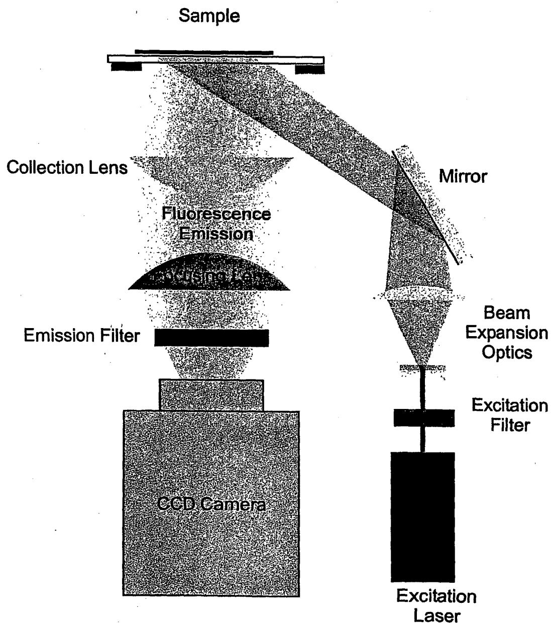
Figure 4. A CCD imaging system for non-magnified large area imaging.
