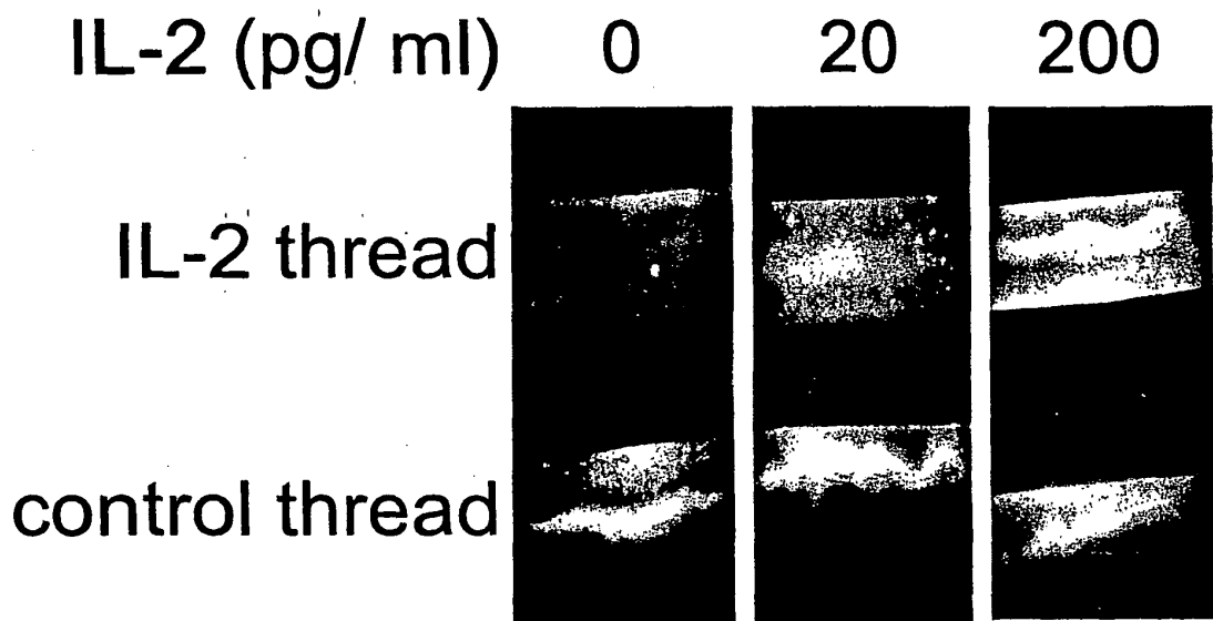
Figure 12. An ultra-sensitive test for a protein using the capture thread format (Example 8).
