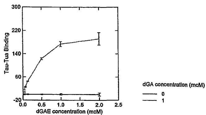
dGA-dGAE Binding
