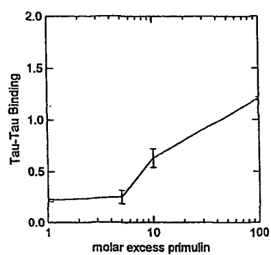
Tau-Tau Binding at 5 mM DMMB
