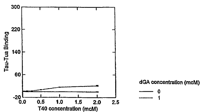
dGA-T40 Binding
