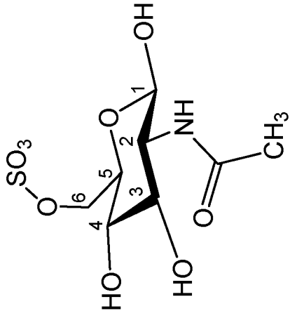
6-Sulfo-N-Acetylglucosamine
