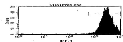
Figure 1: Flow cytometric analysis of control cells
