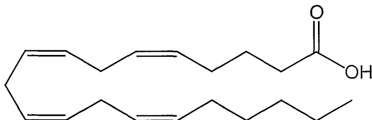
Arachidonic Acid
