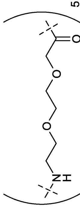
PEG(9-ATOMS) 5
