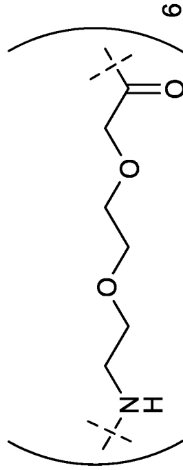
PEG(9-ATOMS) 6
