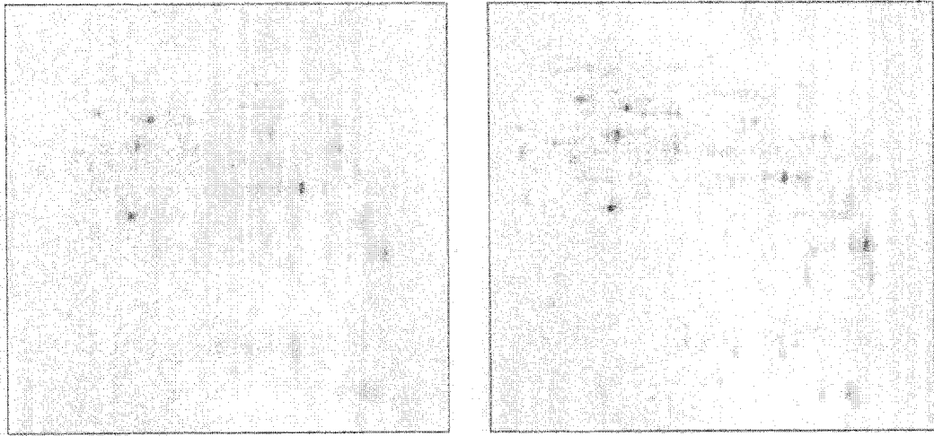
A. Day 1 after Induction of Necrosis
