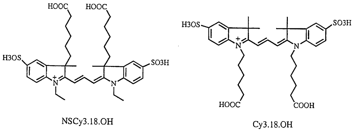
Sulfonated Cy3 dicarboxylic acid isomers
