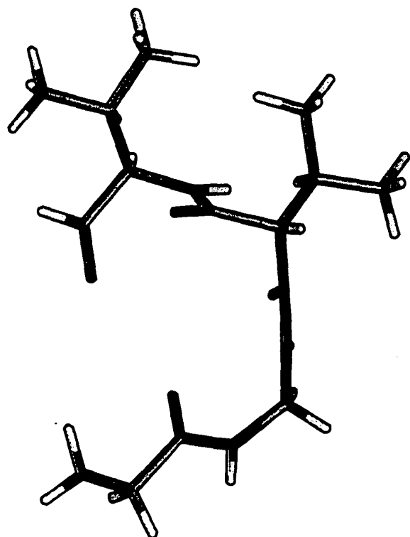
Gly-Gly-CO-NH-Val-Val
