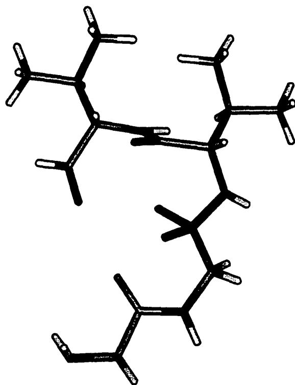
Gly-Gly-PO 2 -NH-Val-Val
