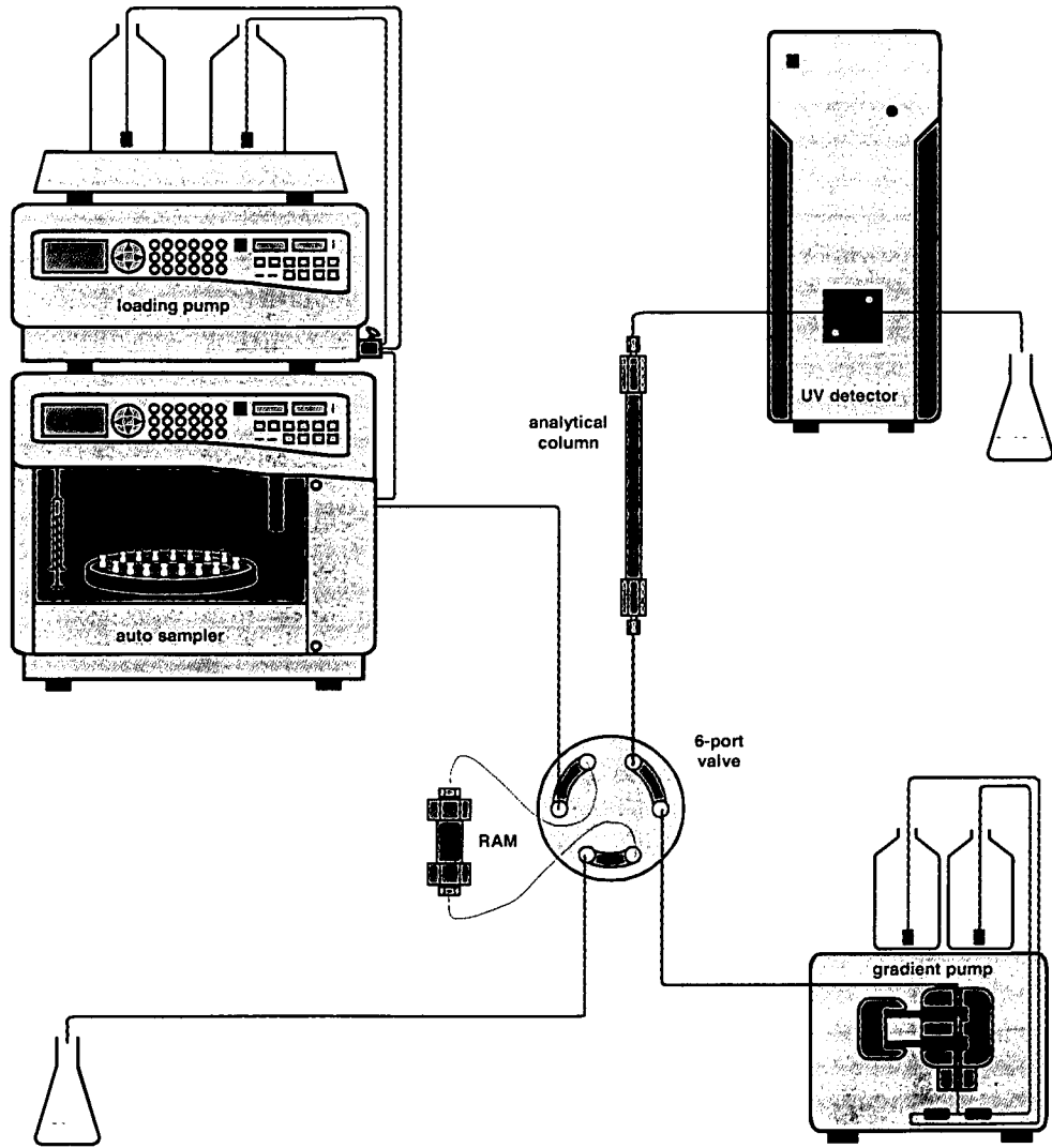
Figure 1: Analytical HPLC setup used to extract immunosuppressives from real blood hemolysates.
