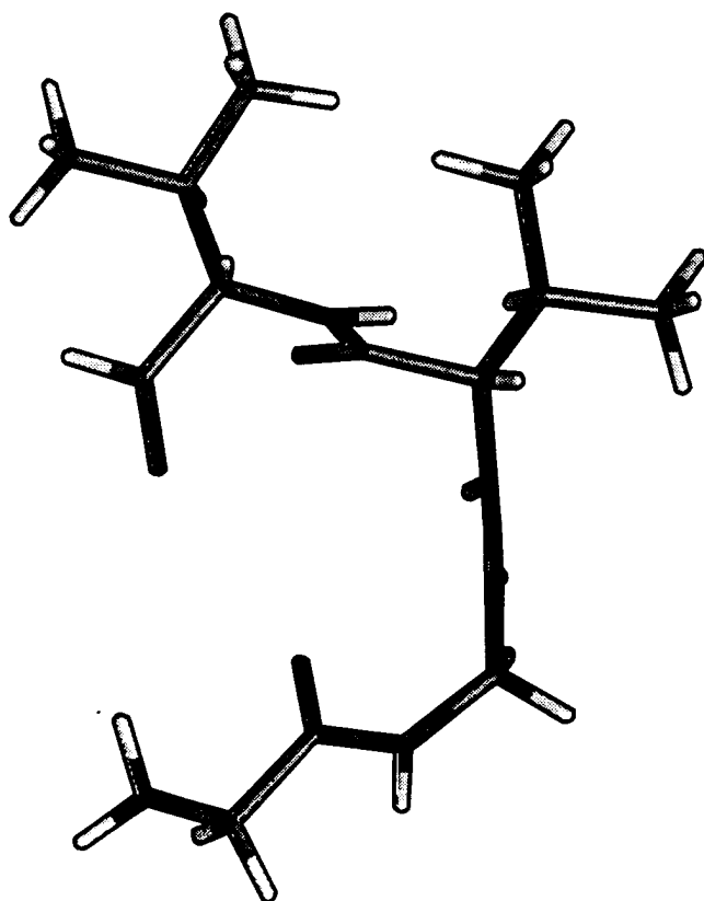
Gly-Gly-CO-NH-Val-Val
