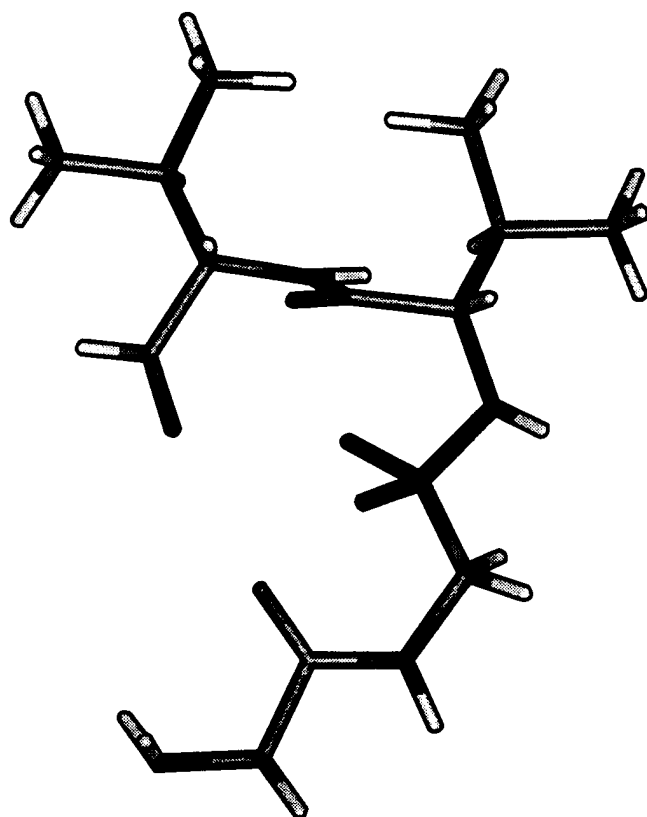
Gly-Gly-PO 2 - -NH-Val-Val
