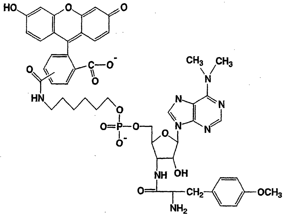
Fluorpur (I)
