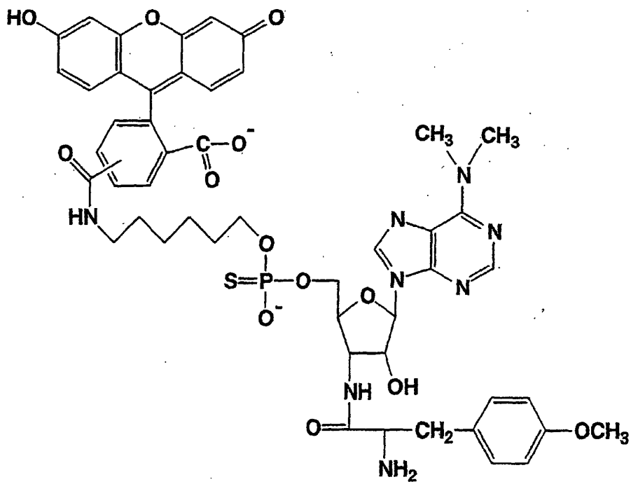
Fluorthiopur (II)
