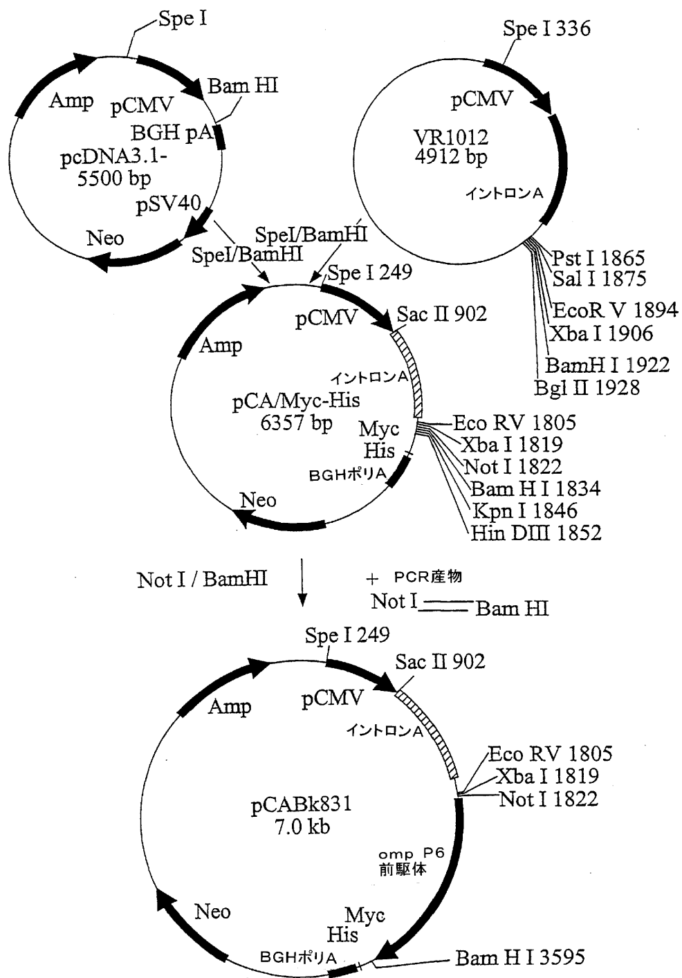
図3: pCABk831の構築
