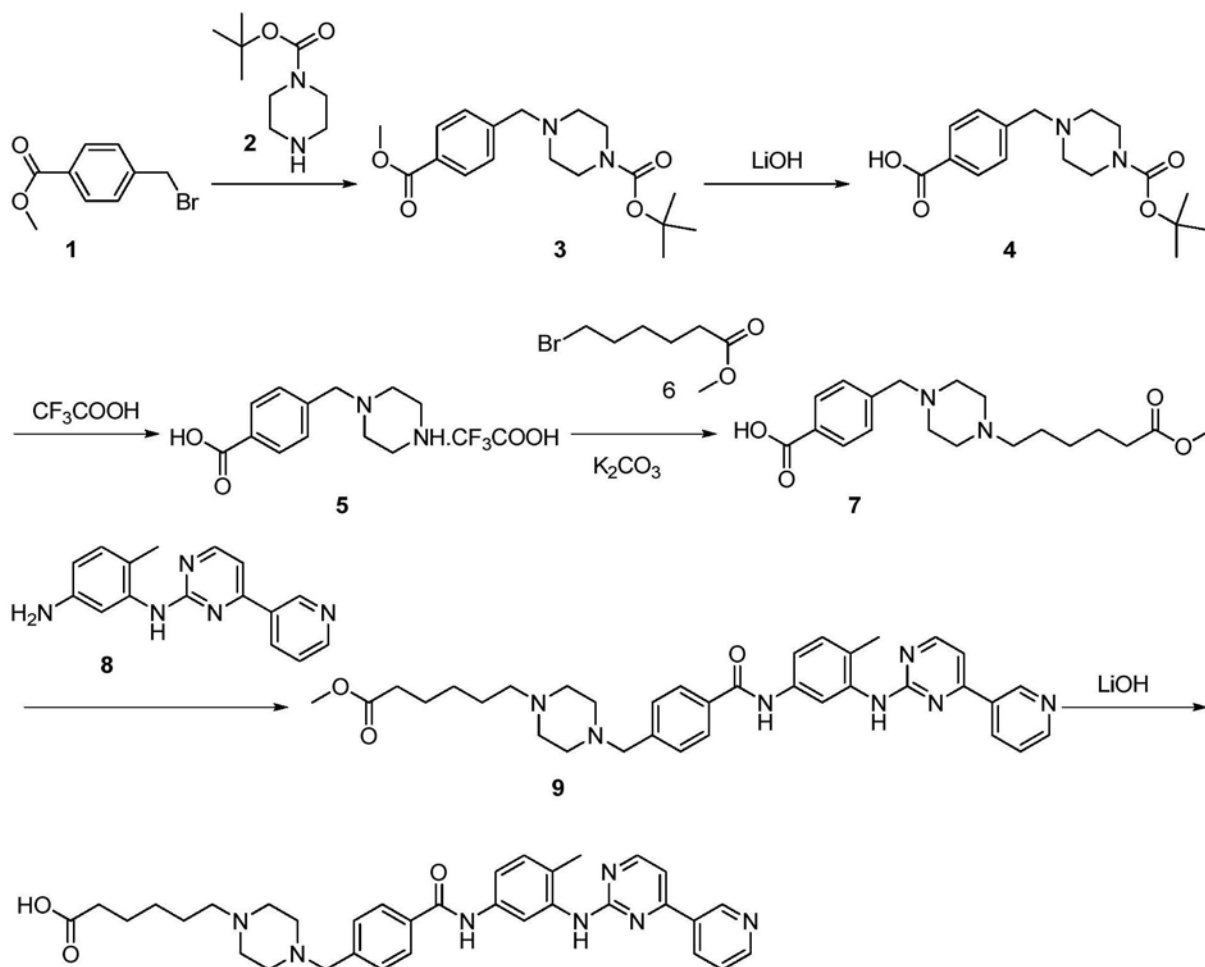
Imatinib Derivative
