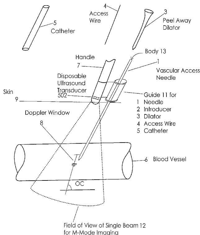
Device for single beam imaging guidance of Vascular Access
