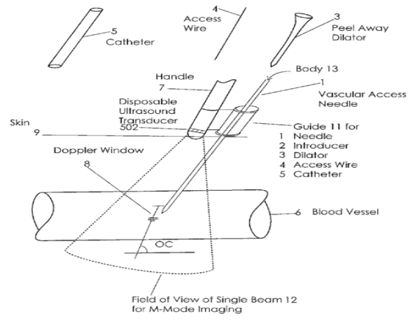
Device for single beam imaging guidance of Vascular Access
