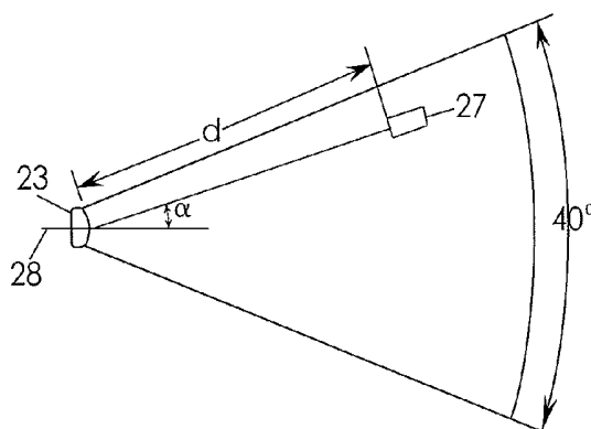
The catheter-based Doppler sensor (27) interacts with the Doppler imaging transducer (23) when it is situated in the transducer's field of view determined by the axis 28, distance d and angle.
