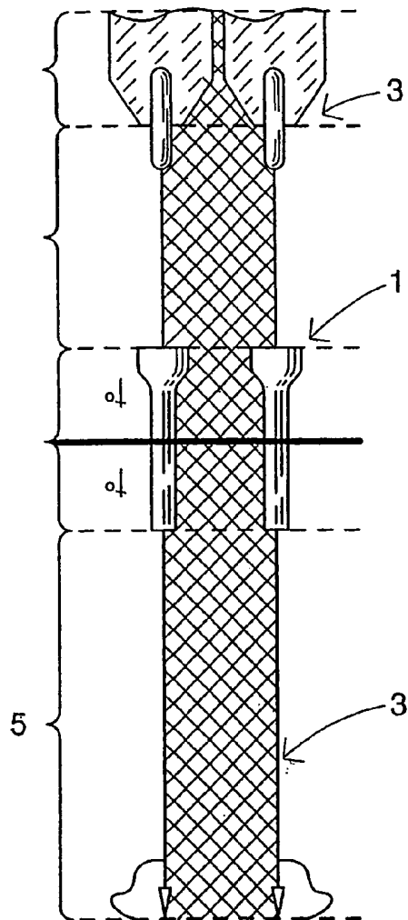
FIG. 1 PRIOR ART
