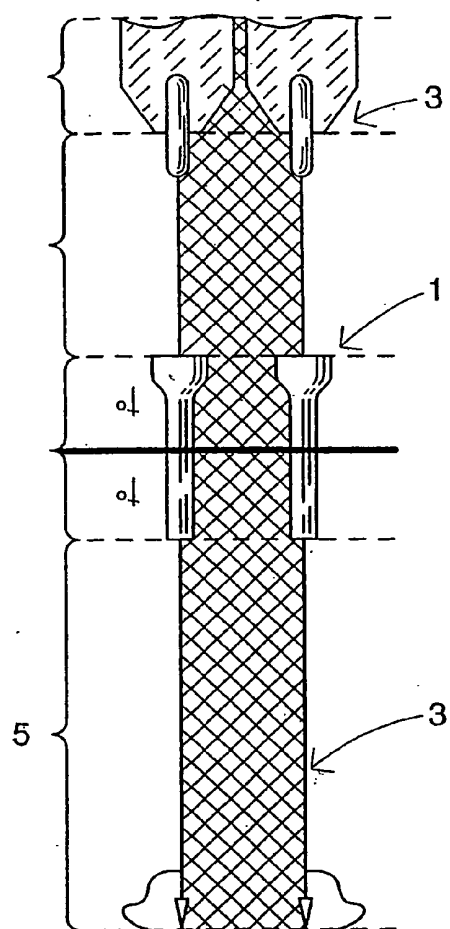
FIG. 1 PRIOR ART
