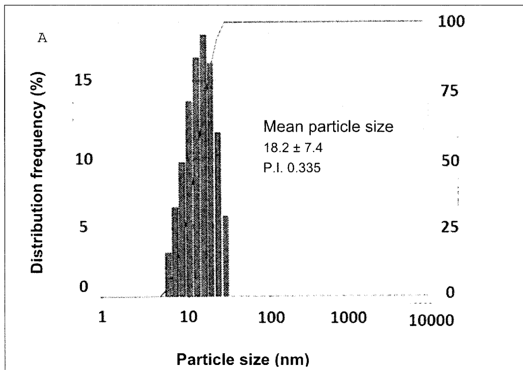
Figure 10-a. Particle size analysis of HPMA-PP.
