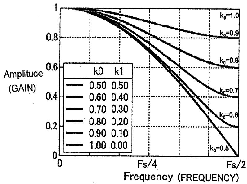
<LPF FREQUENCY CHARACTERISTICS (2-TAP FIR FILTER)>
