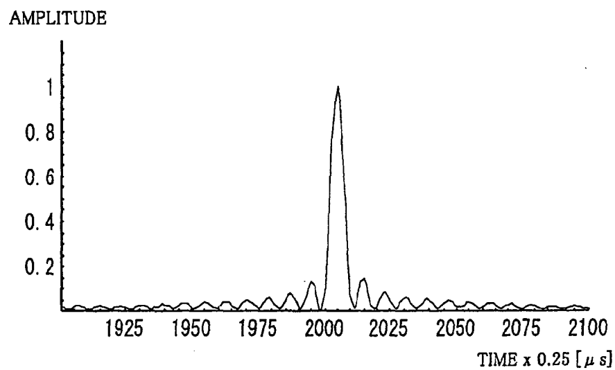
(b) CASE OF 0.5 kHz DOPPLER SHIFT
