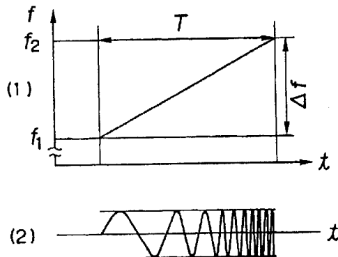
(a) UP CHIRP WAVE (WITHOUT DOPPLER)
