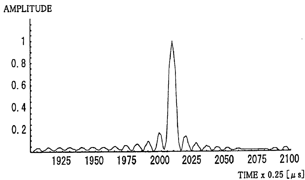
(b) CASE OF 0.5 kHz DOPPLER SHIFT
