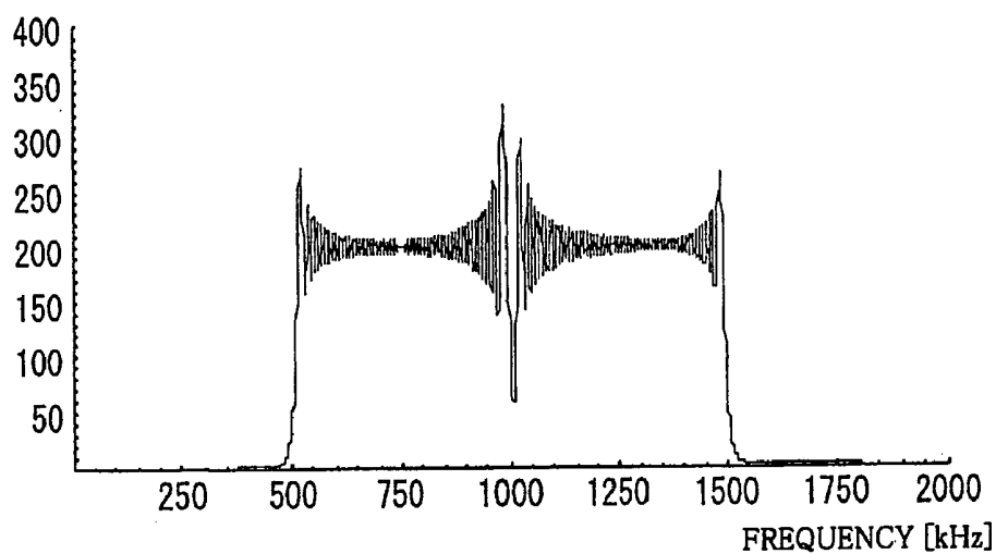
(a) MULTIPLEXED UP CHIRP SIGNAL SPECTRUM
