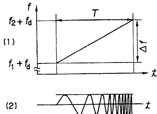
(b) UP CHIRP WAVE (WITH DOPPLER)
