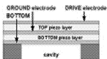
(FIG. 6b) 5V Applied to the DRIVE electrode
