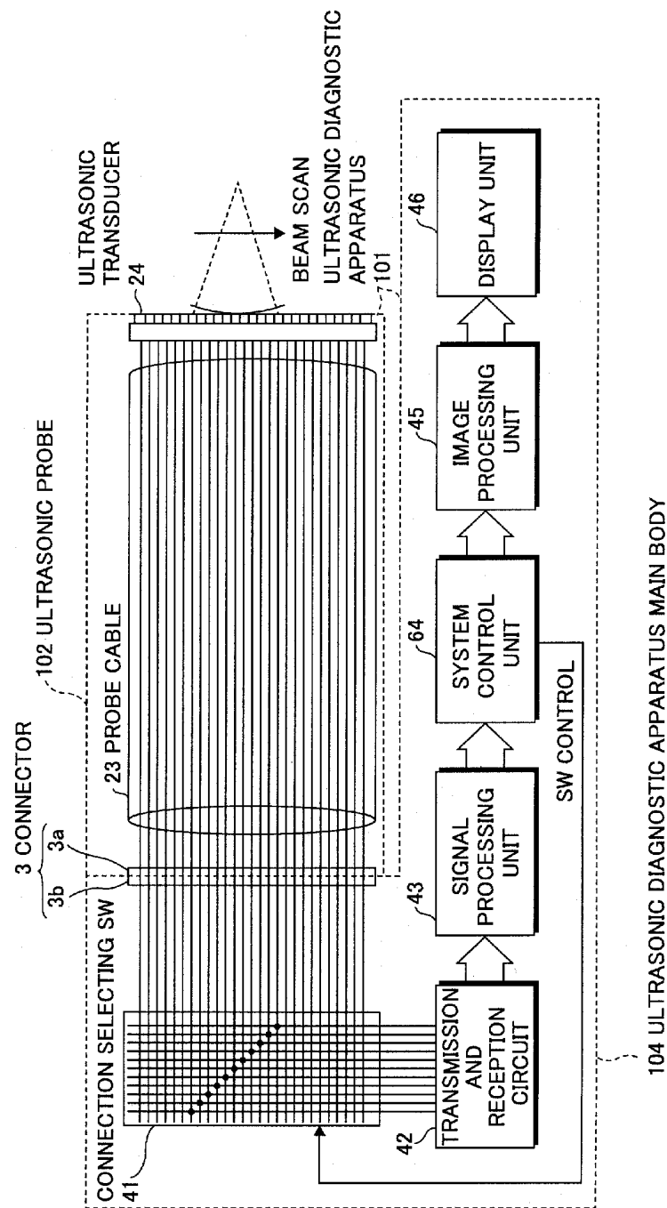
FIG. 7 PRIOR ART
