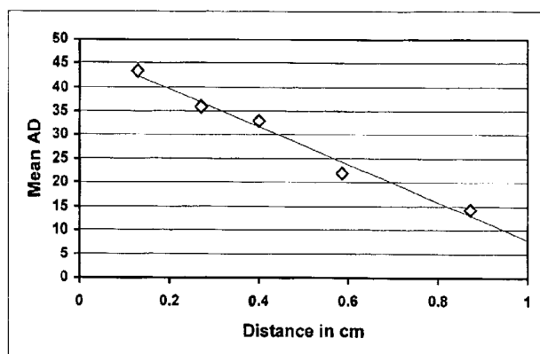
Mean Backscatter AD along Flow Phantom @ MI=1.6
