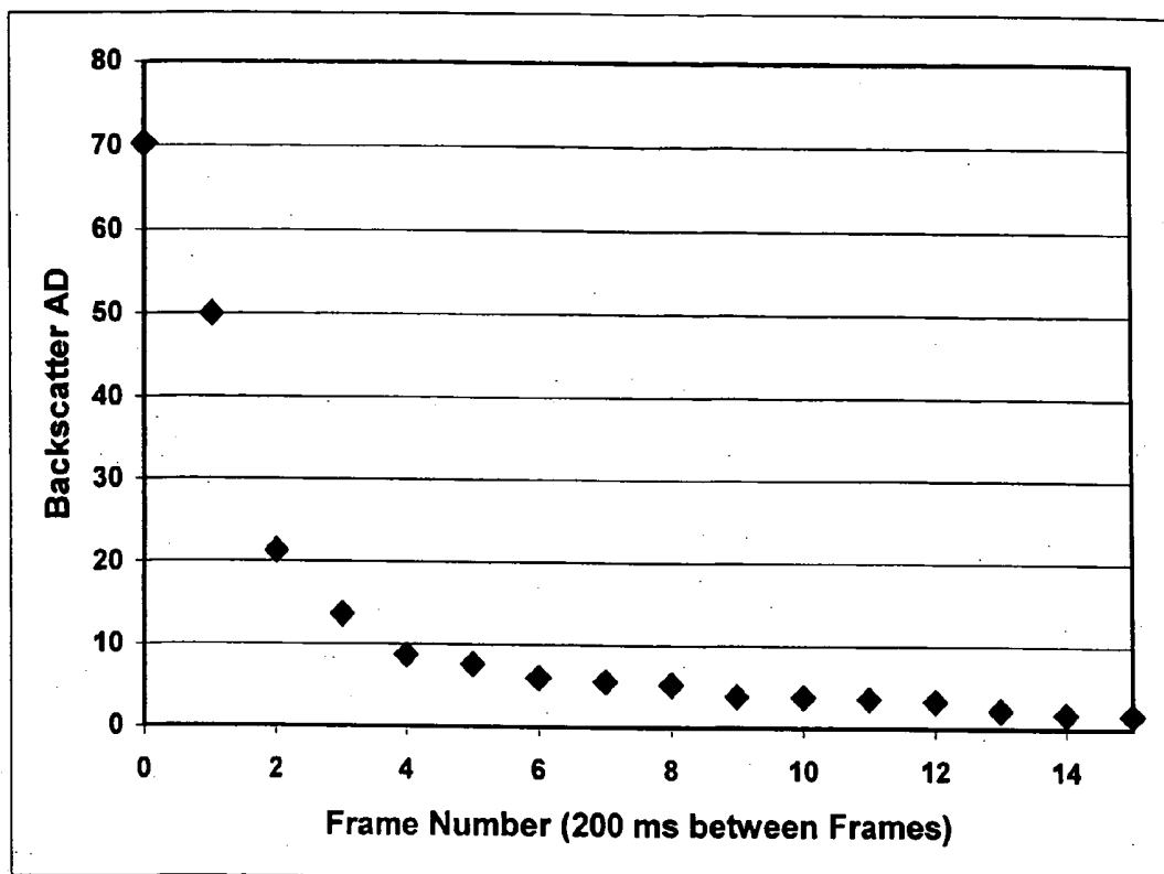
Figure 3. Averaged Backscatter AD Decay Measured Over Sequential Frames @ MI = 1.6
